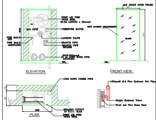
TYPICAL DETAIL OF FIRE HOSE CABINET SIZE (900X600X2100MM) FOR INTERNAL HYDRANT SCALE= N.T.S.
